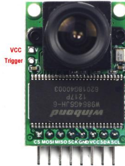
Figure 2 Hardware Trigger Pins
